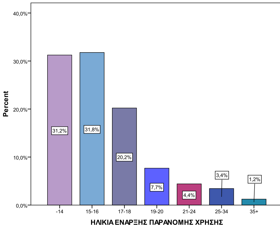
Descriptive Statistics
