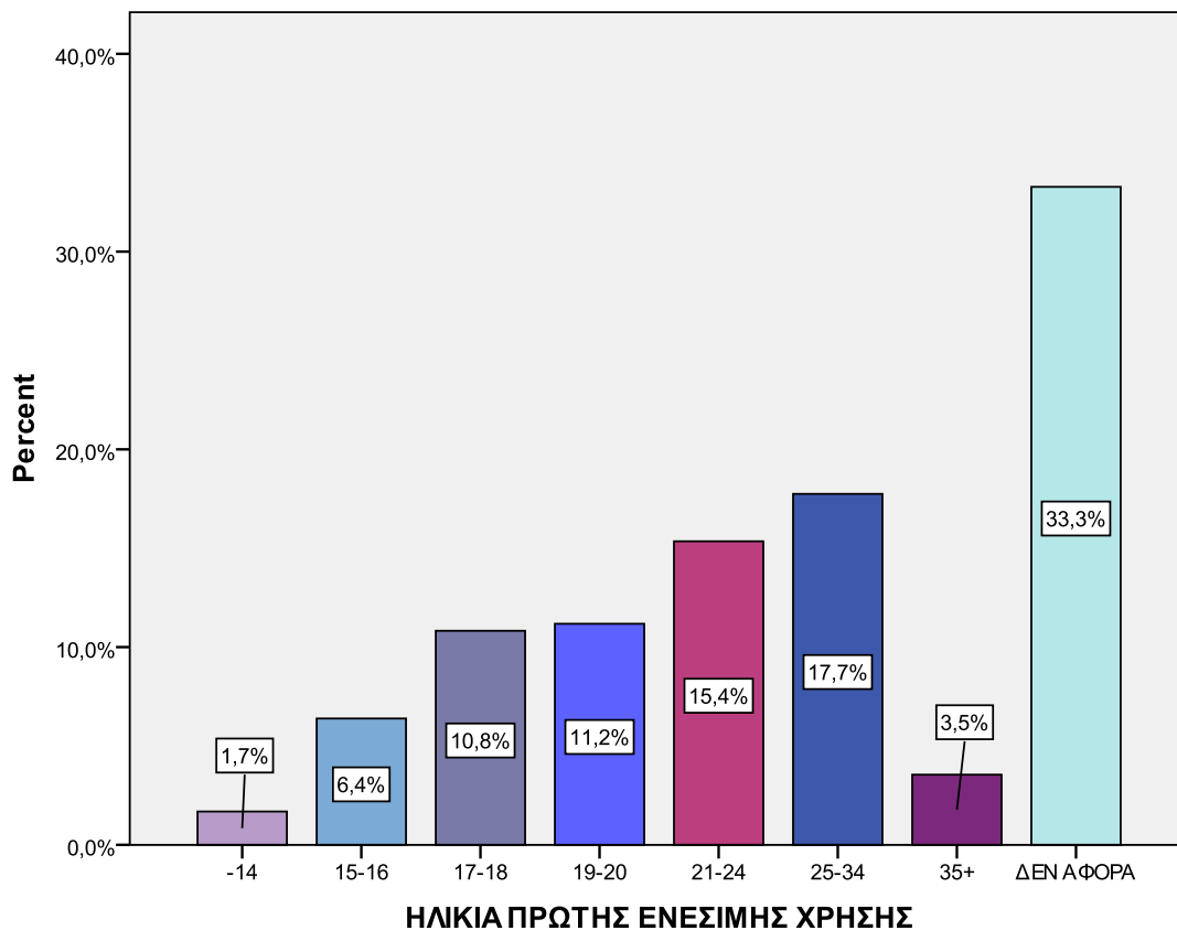
Descriptive Statistics
