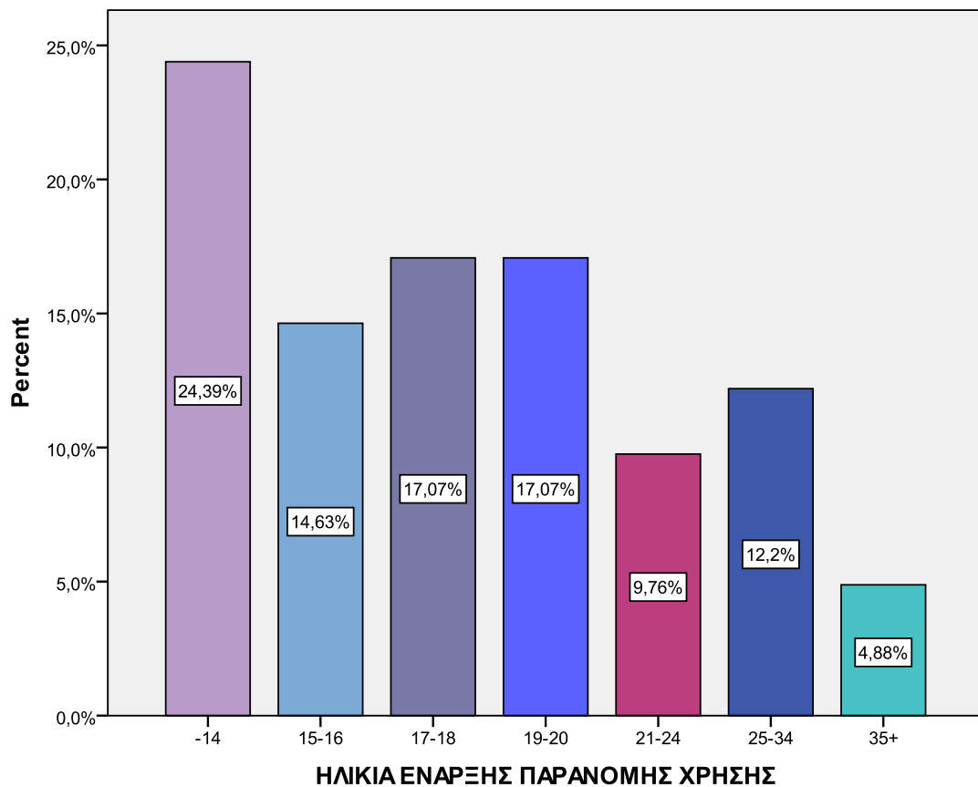
Descriptive Statistics
